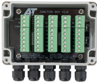
Sealed junction box
