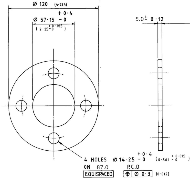
ITEM B WASHER
