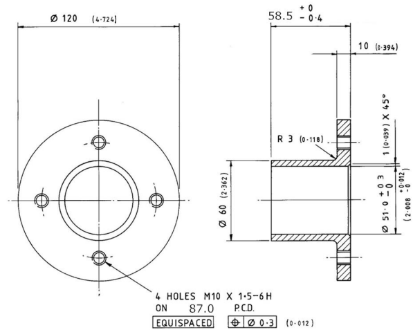
'A' FLANGED BOSS MATERIAL TO MATCH HULL
