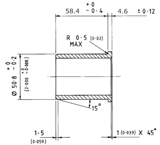
ITEM C BUSH
