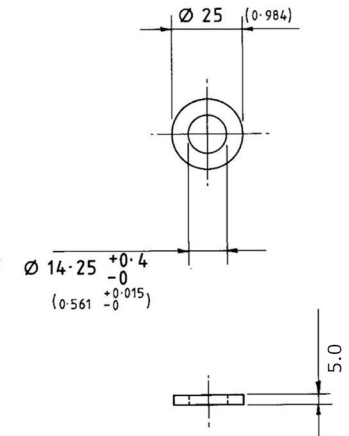
ITEM E WASHER
