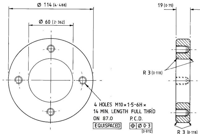
'J' MOUNTING RING
